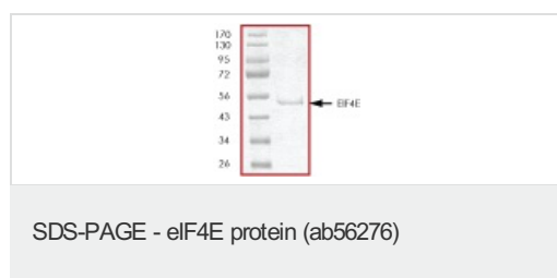
SDS Page analysis of ab56276
