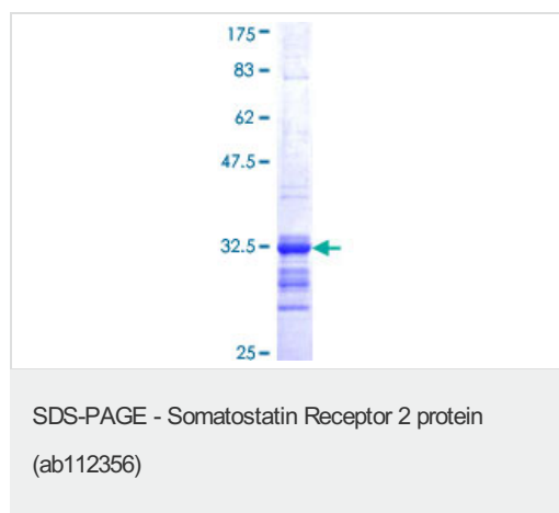
ab112356 on a 12.5% SDS-PAGE Stained with Coomassie Blue.
