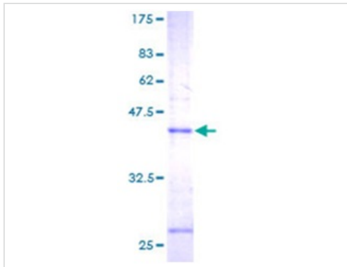
ab114792 on 12.5% SDS-PAGE Stained with Coomassie Blue.
