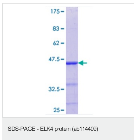
12.5% SDS-PAGE analysis of ab114409 stained with Coomassie Blue.
