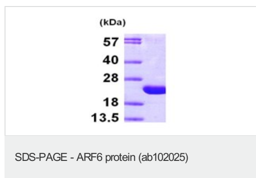
15% SDS-PAGE analysis of ab102025 (3µg)
