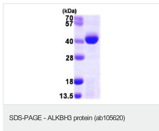
15% SDS-PAGE analysis of ab105620 (3µg)
