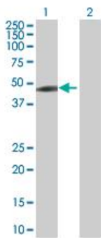
Western blot - Nck 293T Transfected Lysate - (positive control) (ab94184)
