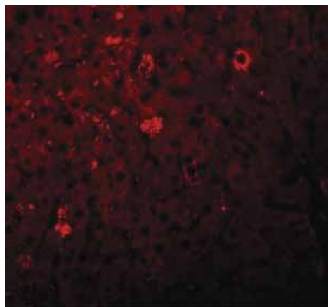
Immunofluorescence of LYRM1 in rat liver tissue with ab106665 at 20 µg/mL.
