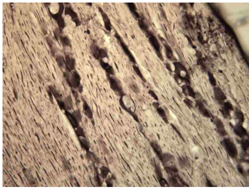
Immunohistochemistry (Frozen sections) - ATP13A2 antibody (ab43074)
